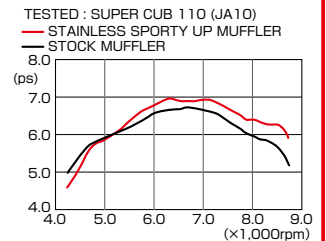
* Tested at Kitaco facility. Actual run may differ * All the other parts except muffler is stock parts.
