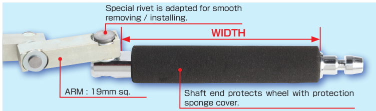
TDZ-05 SHAFT END & ARM
