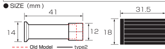
Short rubber type M6 pedal bar type 2 is newly released.
