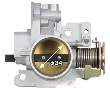
BIG THROTTLE BODY (STOCK : φ 24)
