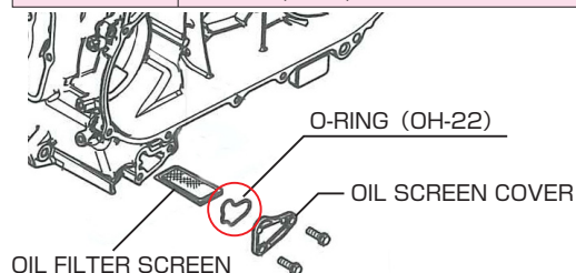
Stock size O-ring. Exchange when leakage and bleeding
