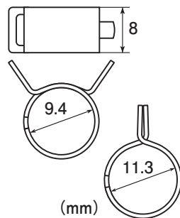
Small size crescent clamp for hose such as \phi 9.4 ~ \phi 11.3 !!
