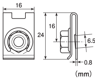
Clip nut for M5 / P0.8 released /
