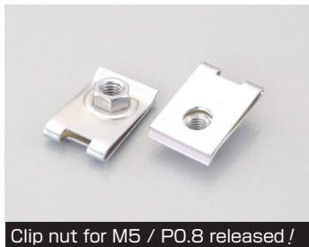
Clip nut for M5 / P0.8 released /
