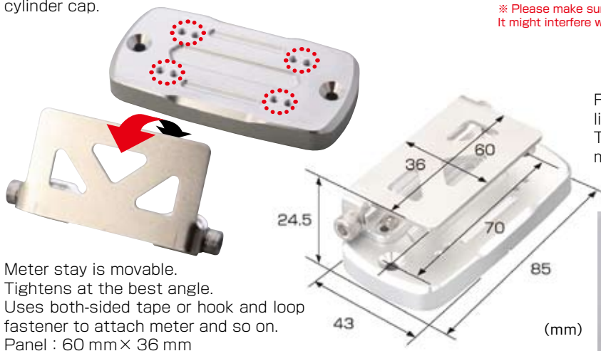
Type 3 has movable meter stay on the top. Angle adjustable for the best meter position.
