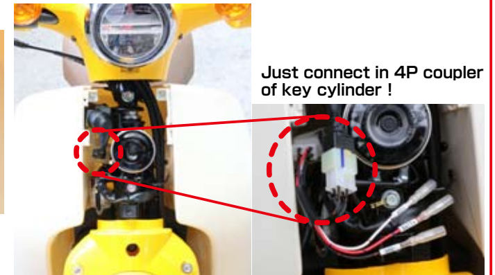
Uses accessory battery (ACC+). It turns on when key is on. Built-in blue LED turns on.
