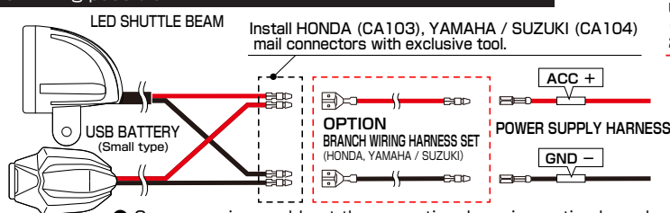
Option branch wiring harness for Kitaco power supply harness. 2 branch wiring possible.
