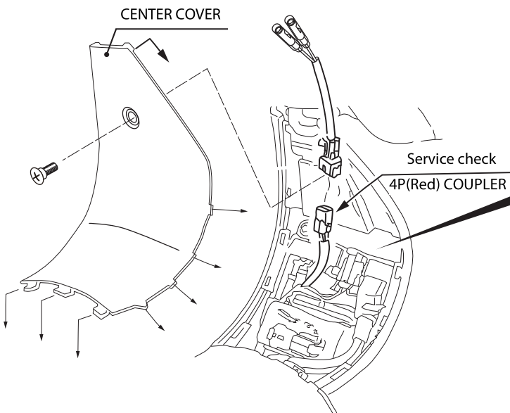
Coupler of inside battery cover
