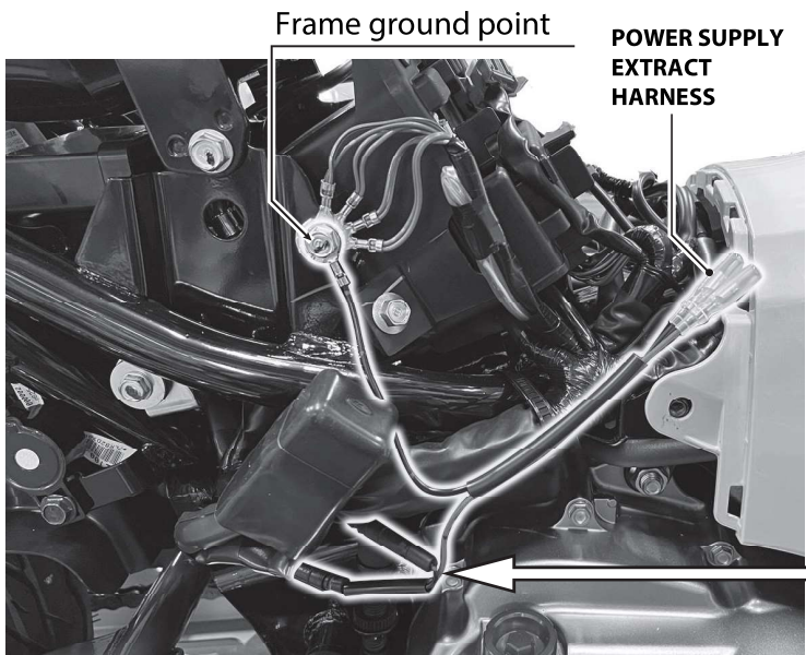
Rear brake light switch connector
